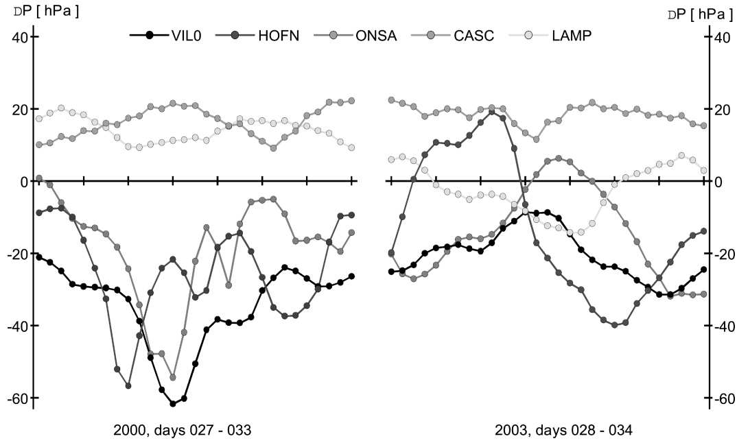
Fig. 6: Pressure anomaly variations at selected sites during two seven days periods
