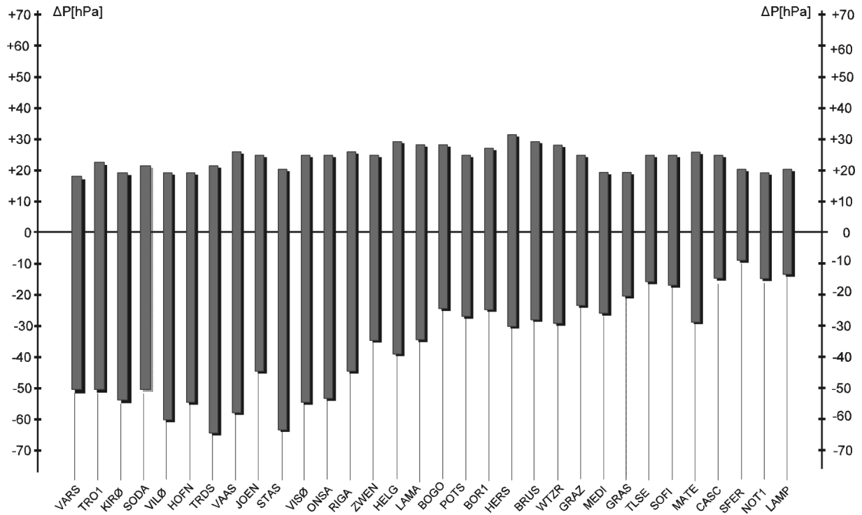
Fig. 4: Range of pressure anomalies at each involved site during the analysed periods
