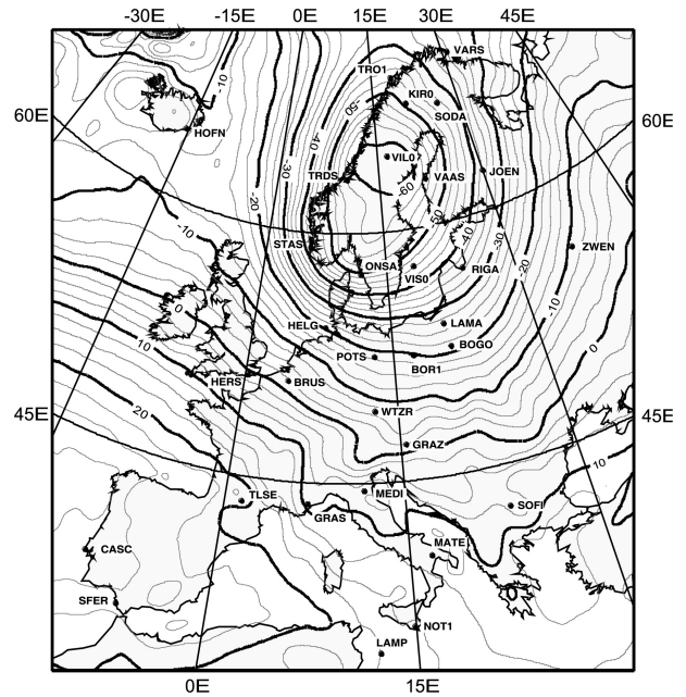
Fig. 3: Pressure anomalies in the network area on January 30, 2000, at 0 hrs UT [hPa]
