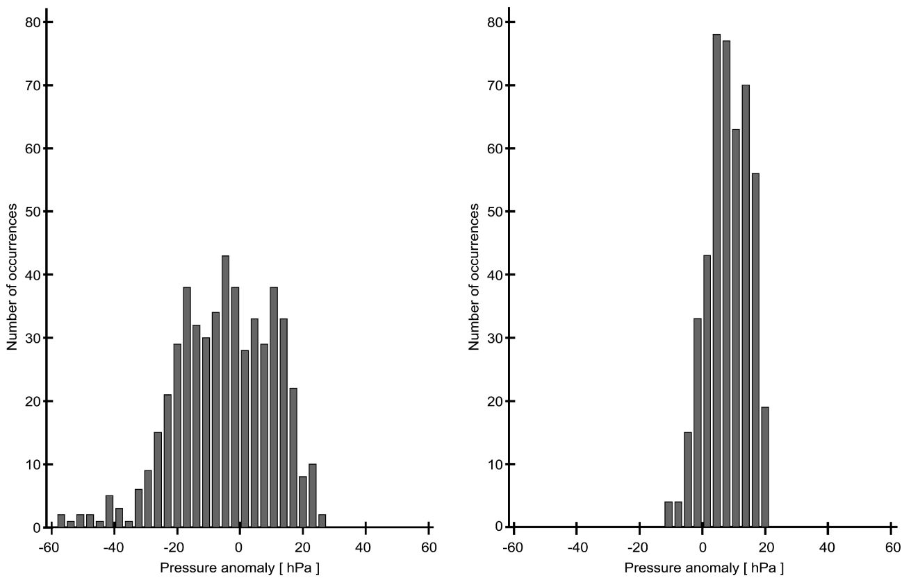
Fig. 5: Distribution of pressure anomalies at VISØ (left) and LAMP (right)
