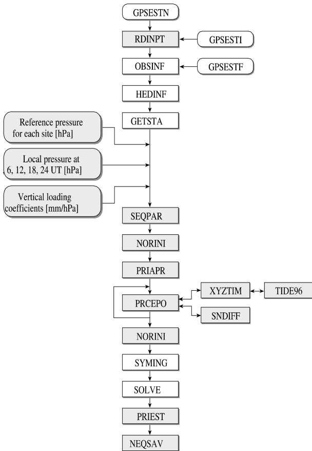
Fig. 1: Generalized flow chart of the Bernese adjustment program GPSEST; modified modules and new data files are underlayed in grey.
