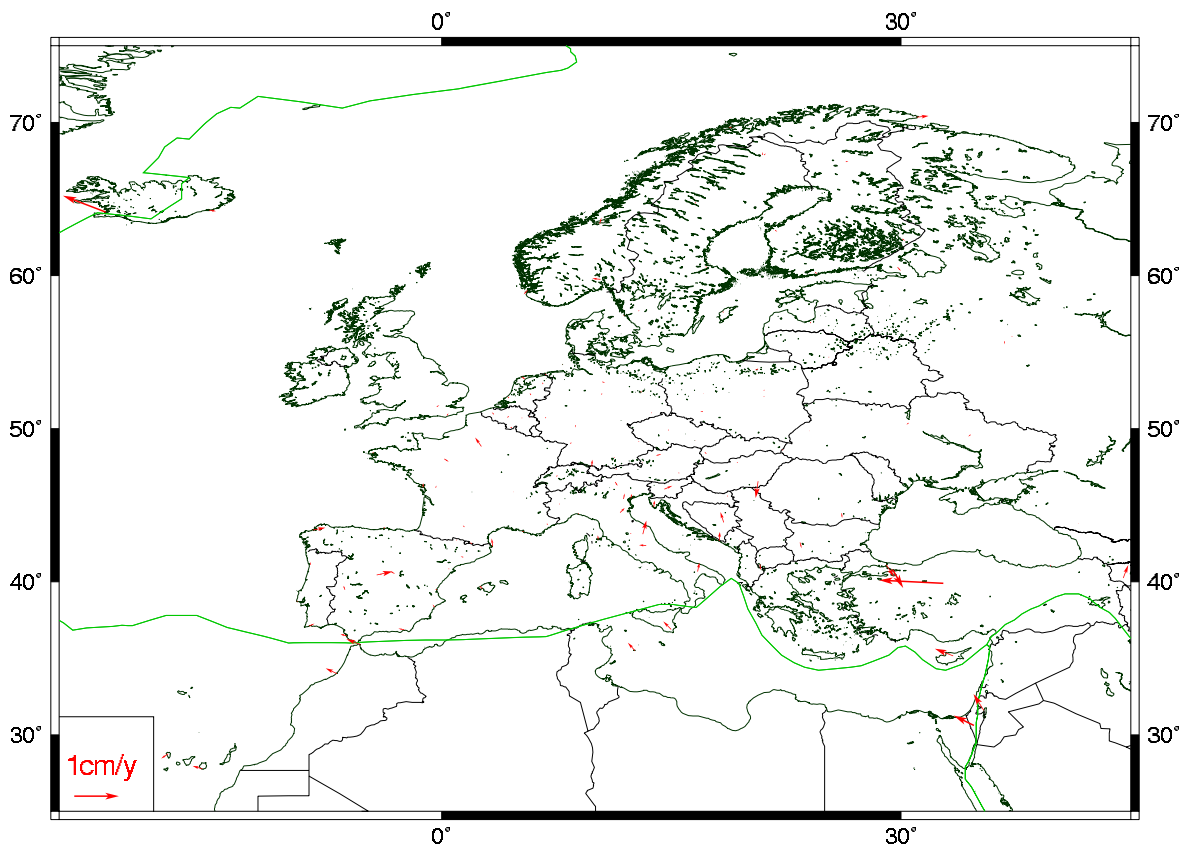
Figure 5. ETRF2000 horizontal velocities of EPN stations.
