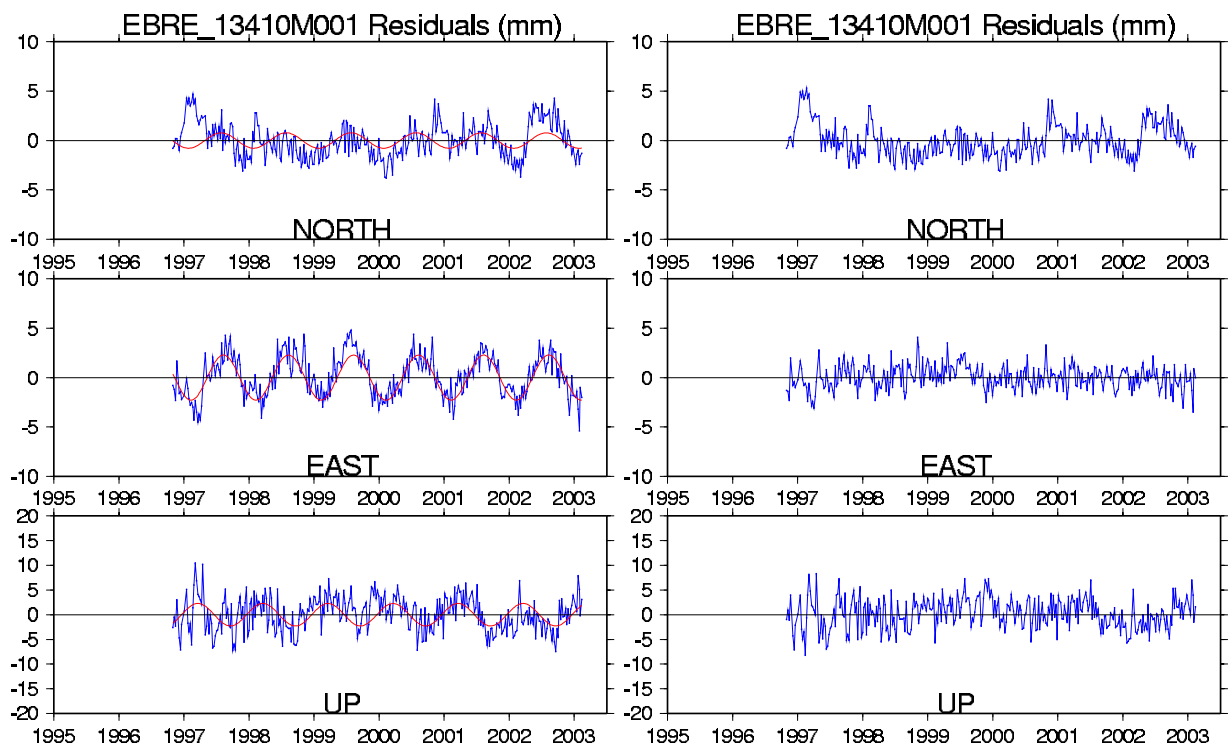
Figure 3. Example of annual variations before and after amplitude and phase modelling.
