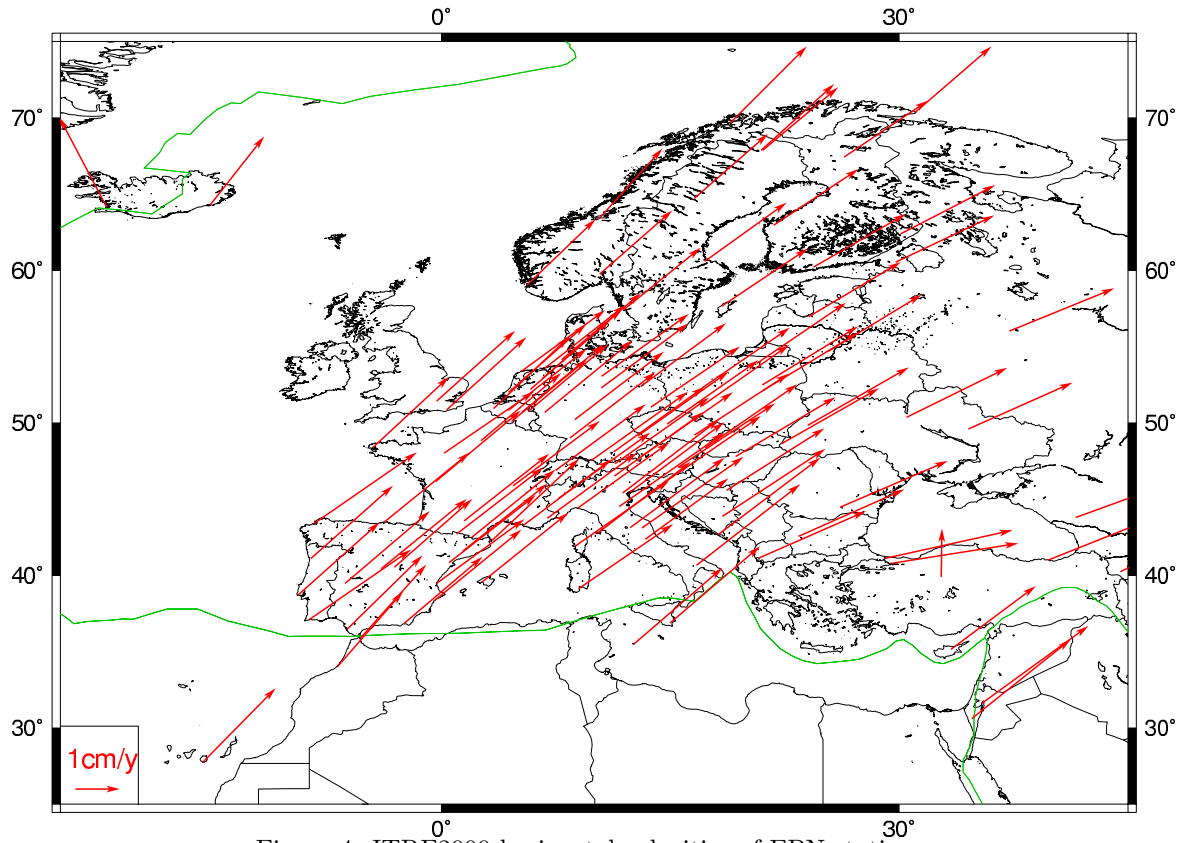
Figure 4. ITRF2000 horizontal velocities of EPN stations.
