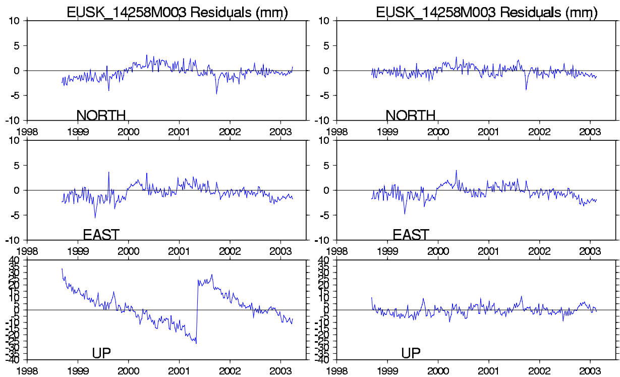
Figure 2. Example of time series discontinuity before and after break-wise modelling.
