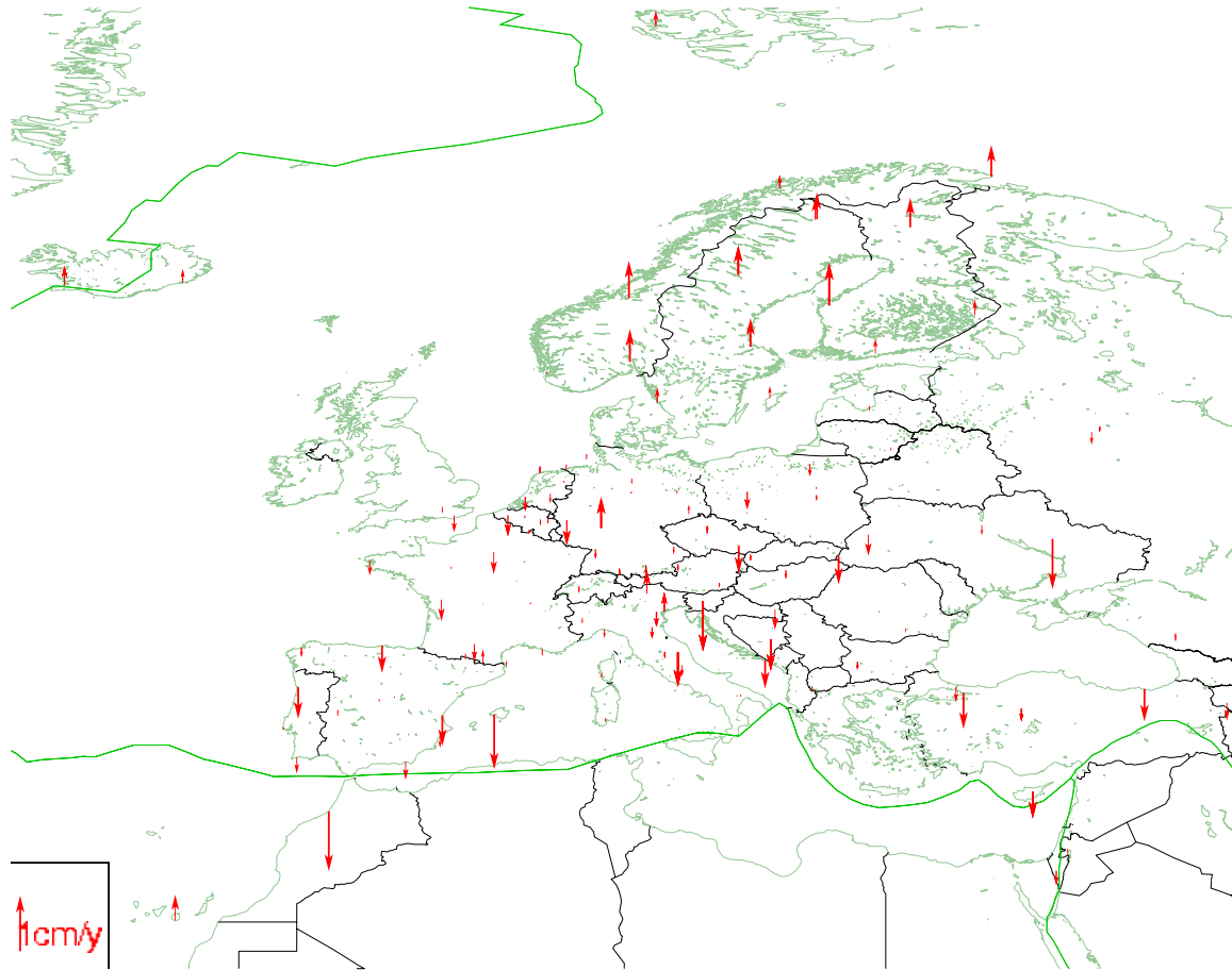
Figure 6. ITRF2000/ETRF2000 vertical velocities of EPN stations.
