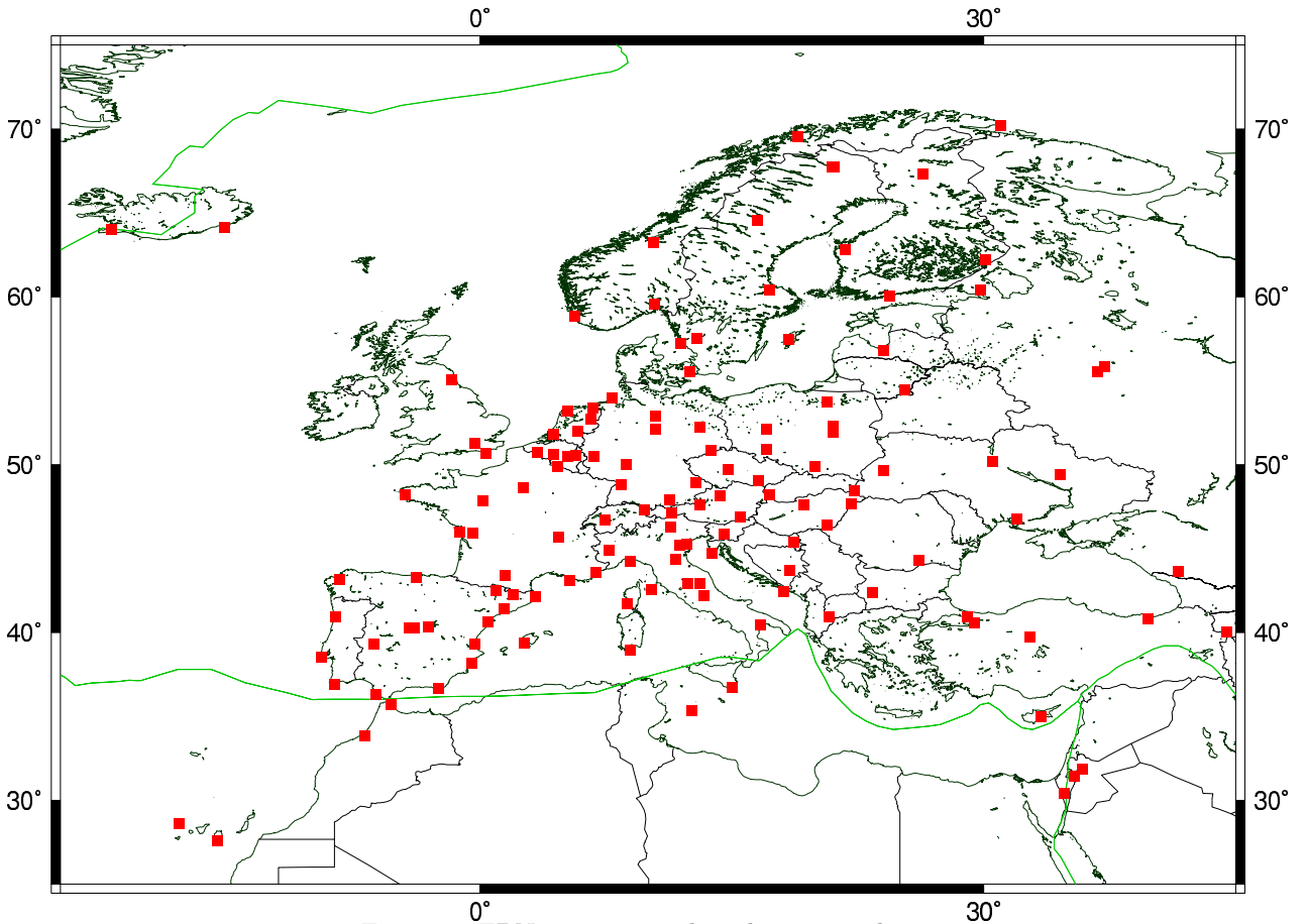
Figure 1. EPN stations used in the test analysis.
