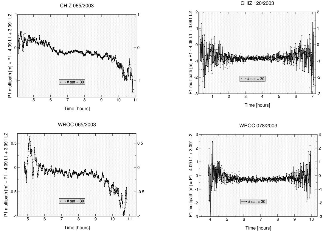
Figure 11 – Left graphs: L1 multipath showing a negative slope due to Ashtech smoothing algorithm; Right: Normal L1 multipath with smoothing turned off.
