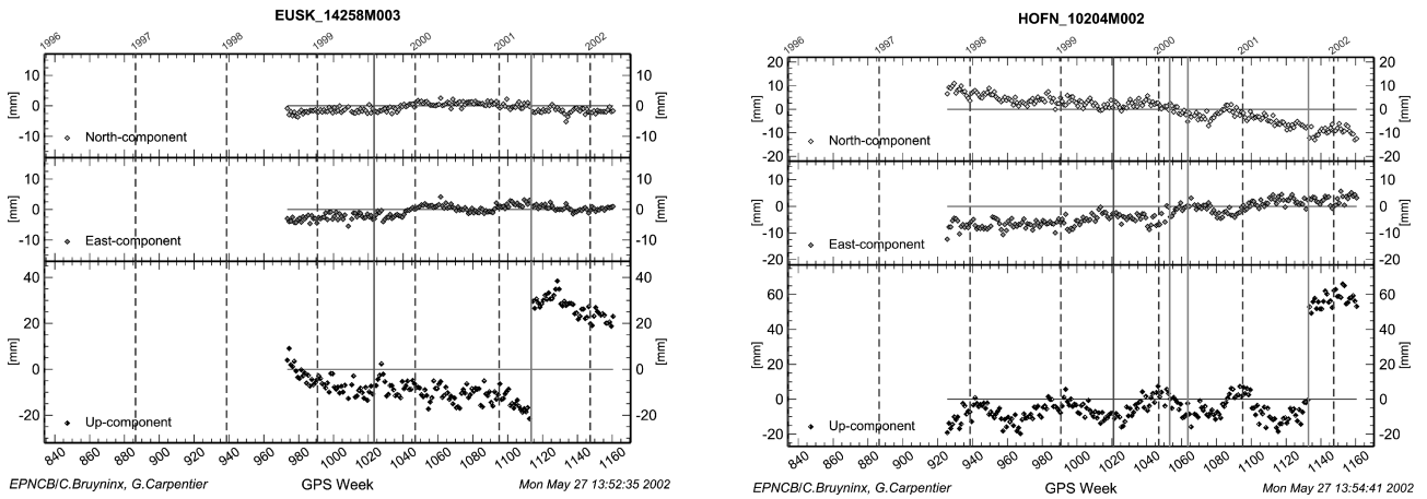
Figure 7: Standard coordinate time series for Euskirchen, Germany (left) and Hofn, Iceland (right)
