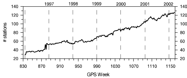
Figure 2: Growth of the EPN Network
