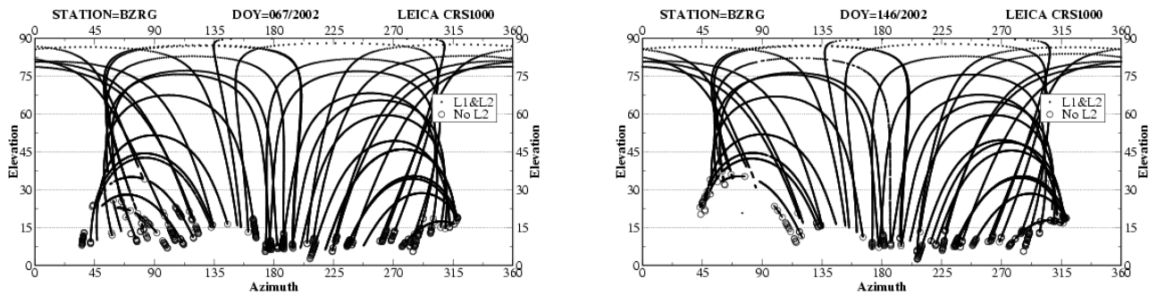
Figure 11: Azimuth/elevation graphs for BZRG. Left: normal tracking (March 2002); Right: degraded tracking with missing data at azimuth around 60 degrees (May 2002)
