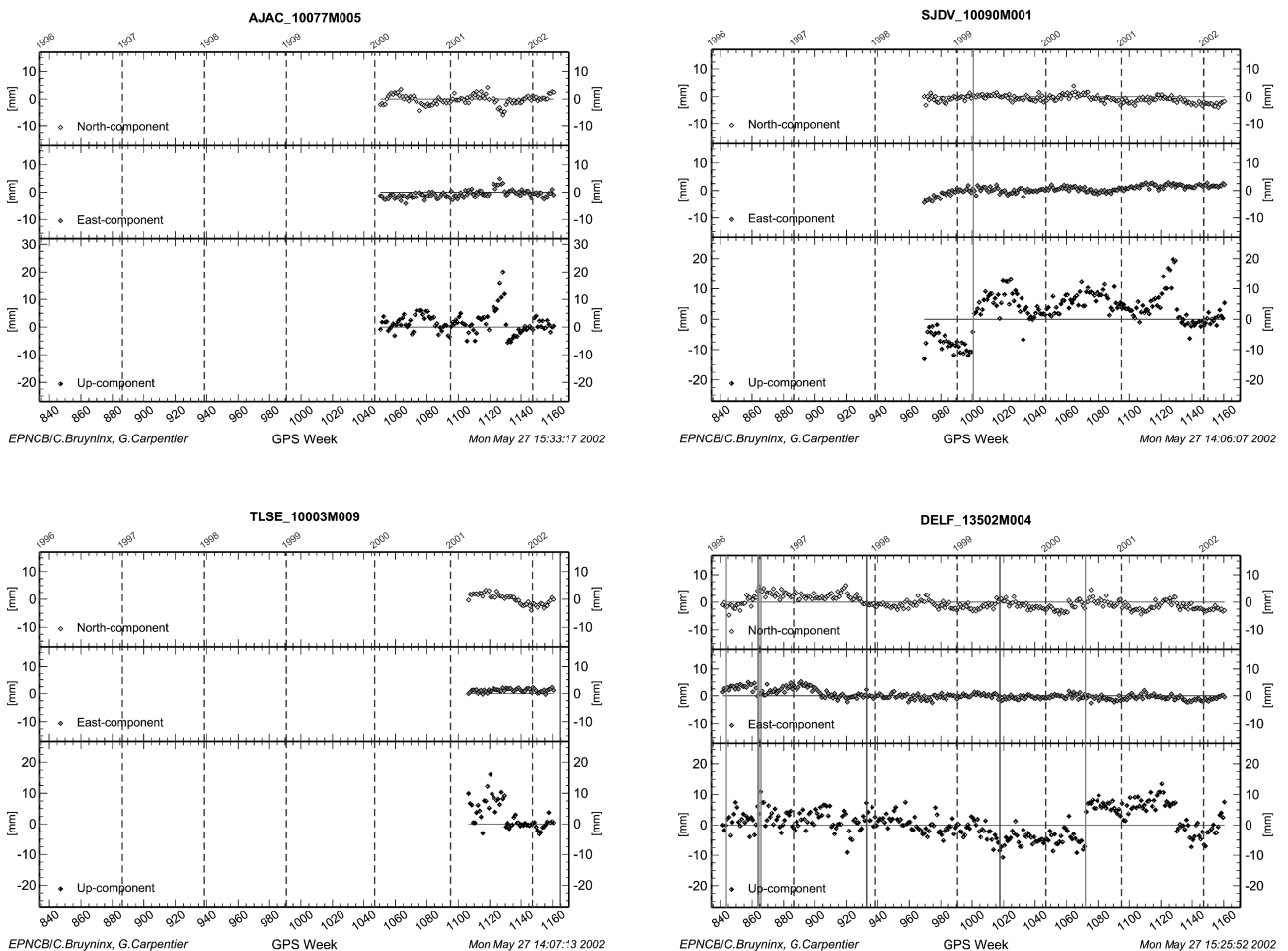
Figure 8: Standard coordinate time series for AJAC (upper left), SJDV (upper right), TLSE (bottom left), DELF (bottom right)
