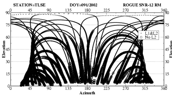
Figure 9: Azimuth/elevation graphs for TLSE. Left: degraded tracking on L2 (April 2002); Right: tracking improvement on L2 after the firmware upgrade (May 2002)
