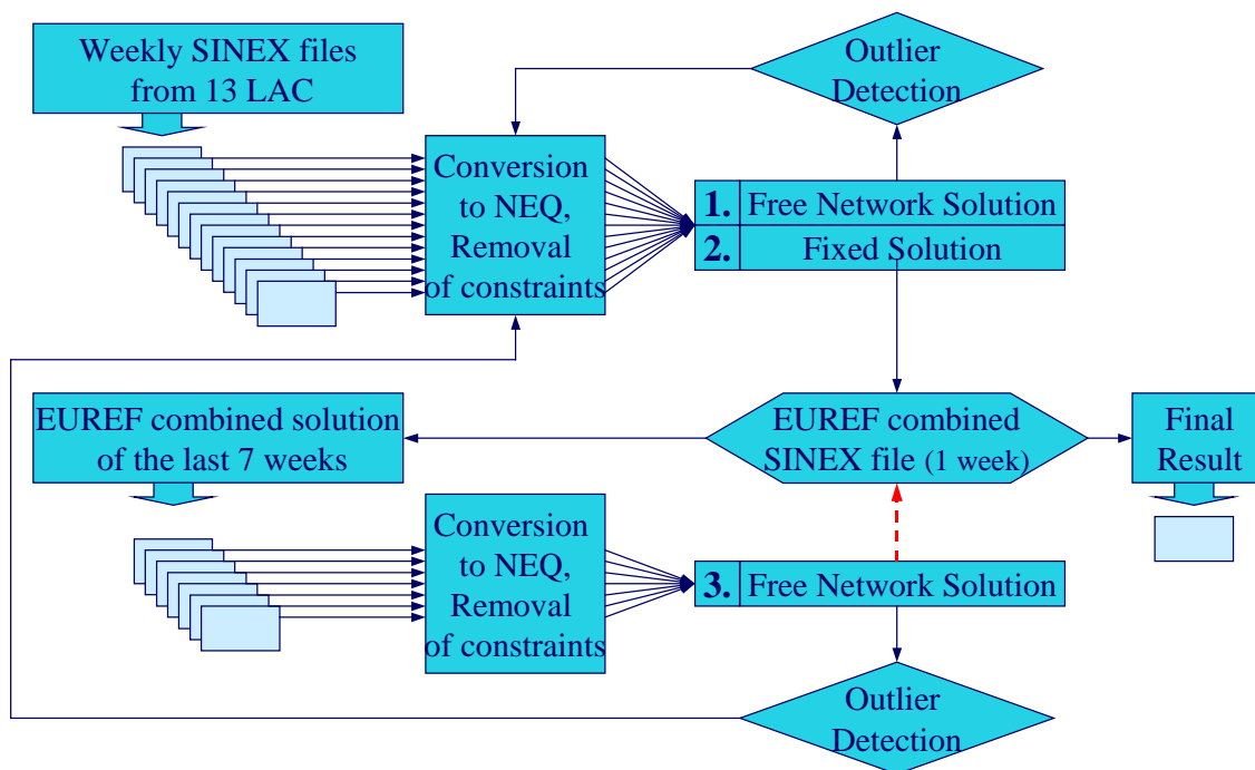
Figure 1: Combination Scheme
