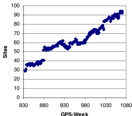
Fig. 1: Growth of the permanent network EPN with time.
