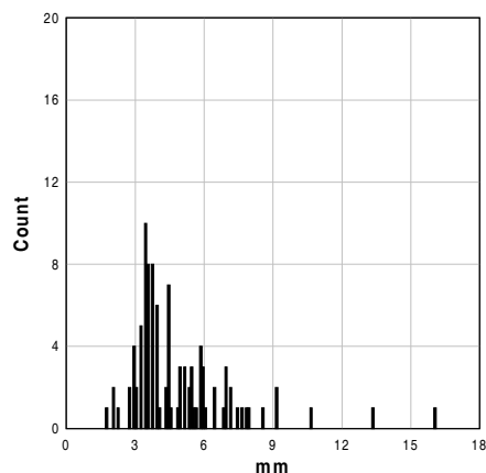
Fig. 4, 5, 6: Residual rms of weekly solution versus the multi year combination.
