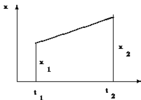
Fig. 3: Modeling of time dependent parameters in ADDNEQ2.
