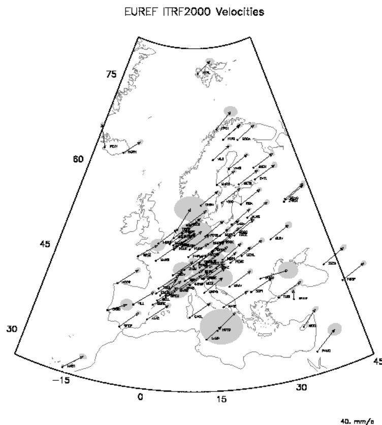
Fig. 7. Velocities of the unconstrained solution for the EUREF contribution to ITRF2000. Formal error ellipses are scaled by a factor of 15 for the plot.
