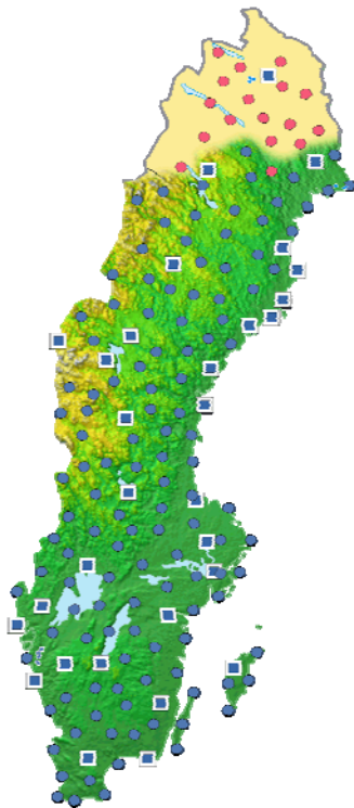
Figure 2: The SWEPOS network in May 2009. Squares are the 32 class A SWEPOS stations. Blue dots are the rest of the existing stations. Red dots are stations that are planned to become operational during 2009.
