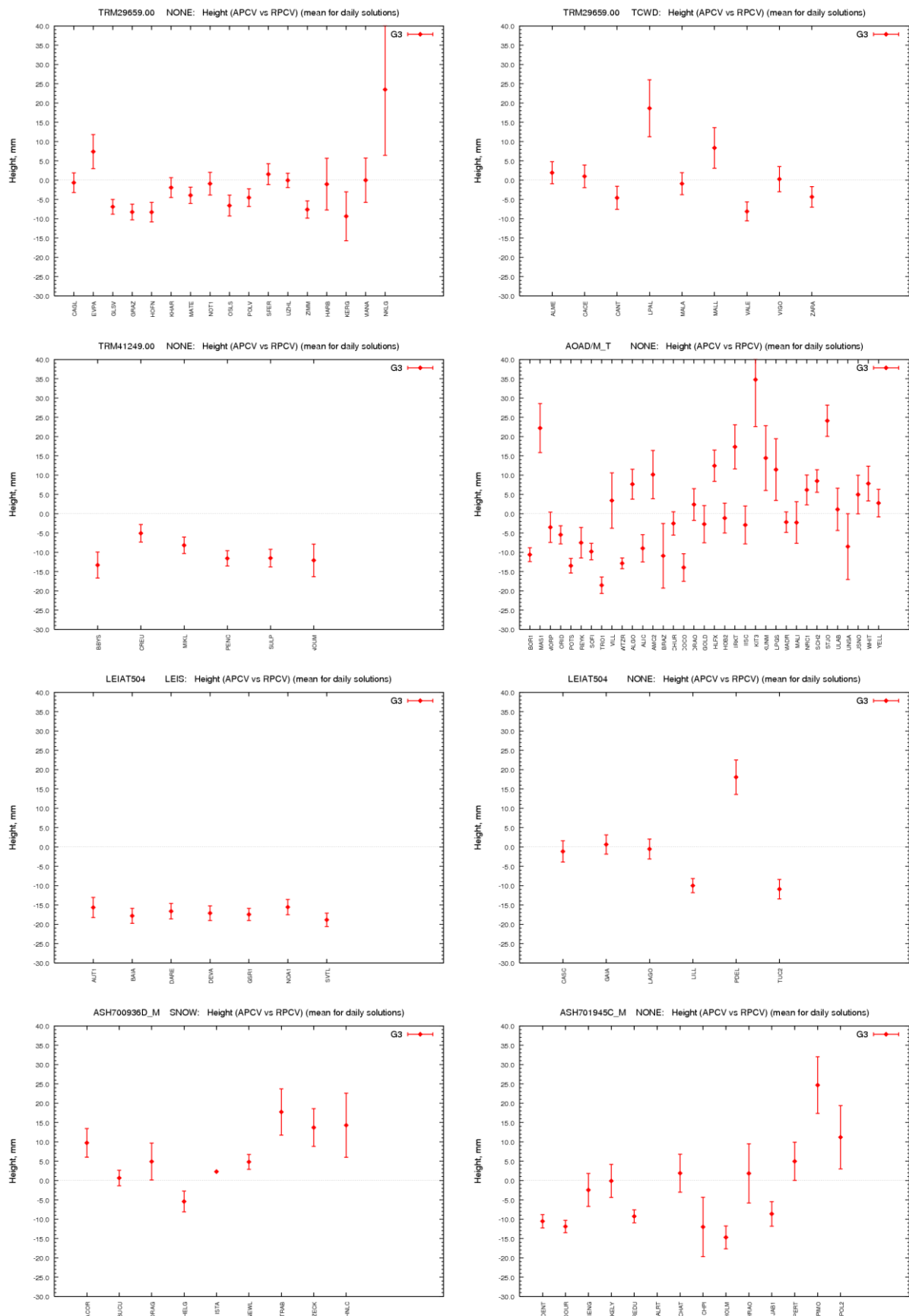
Figure 4 – Mean values of the height residuals of Helmert parameter determination (variant G3)
