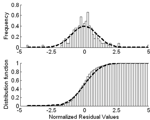
Fig. 5 – Residual Histogram and Normal Probability Plot for Cagliari Super Site and ASI AC. The bold lines are the theoretical values.
