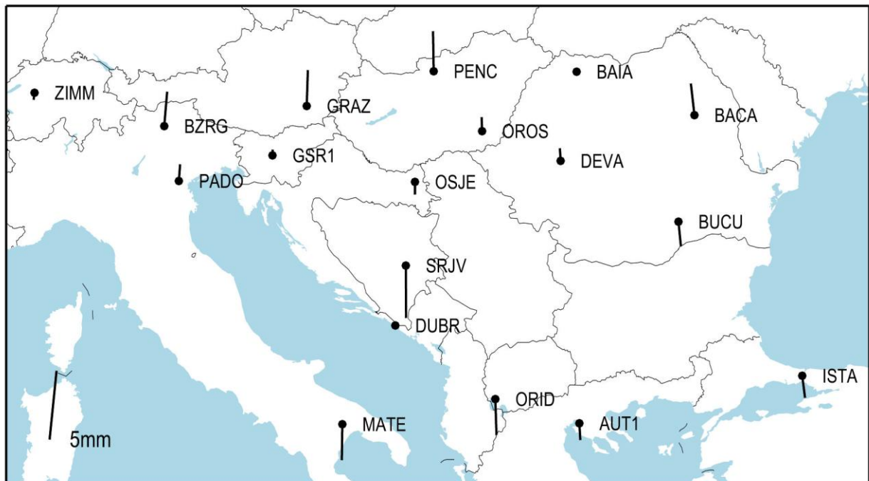
Figure 7. Vertical residuals from fiducial station co-ordinate recoveries
