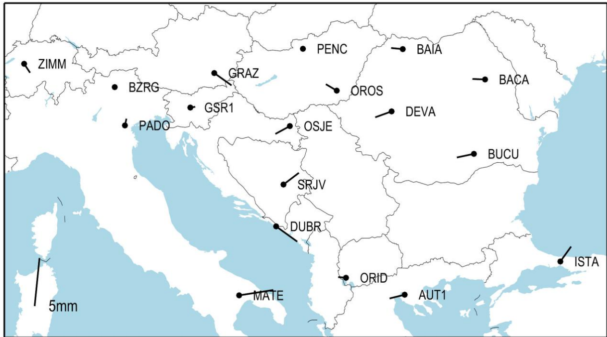
Figure 6. Horizontal residuals from fiducial station co-ordinate recoveries
