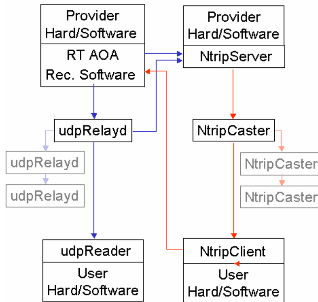
Fig. 2: NTRIP – RTIGS Interface
