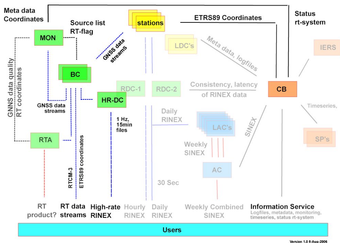
Fig. 1: New EPN Structure
